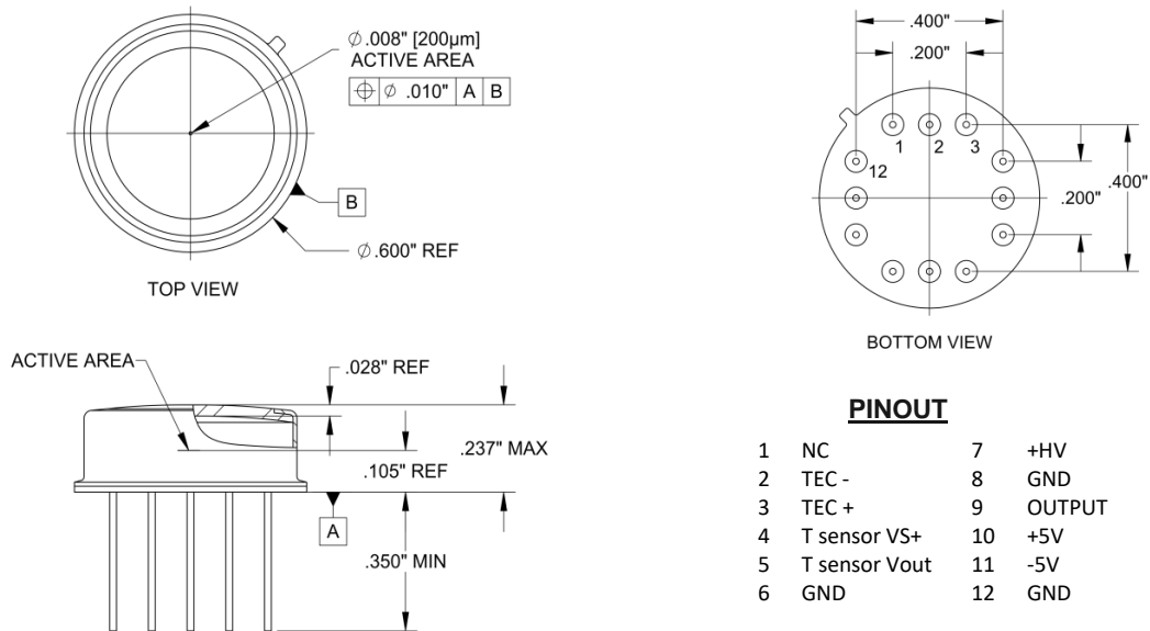
Figure 2: PACKAGE DIMENSIONS & PINOUT
